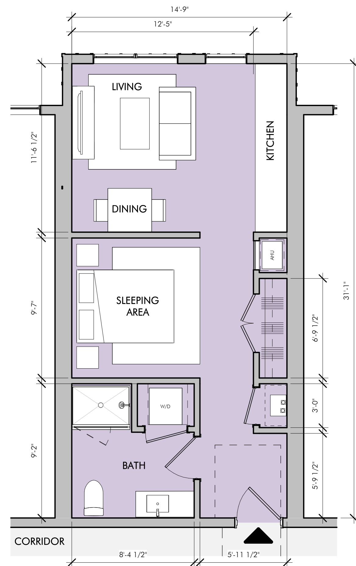
A TYPICAL STUDIO (450 SF) 1/4" = 1'-0"
