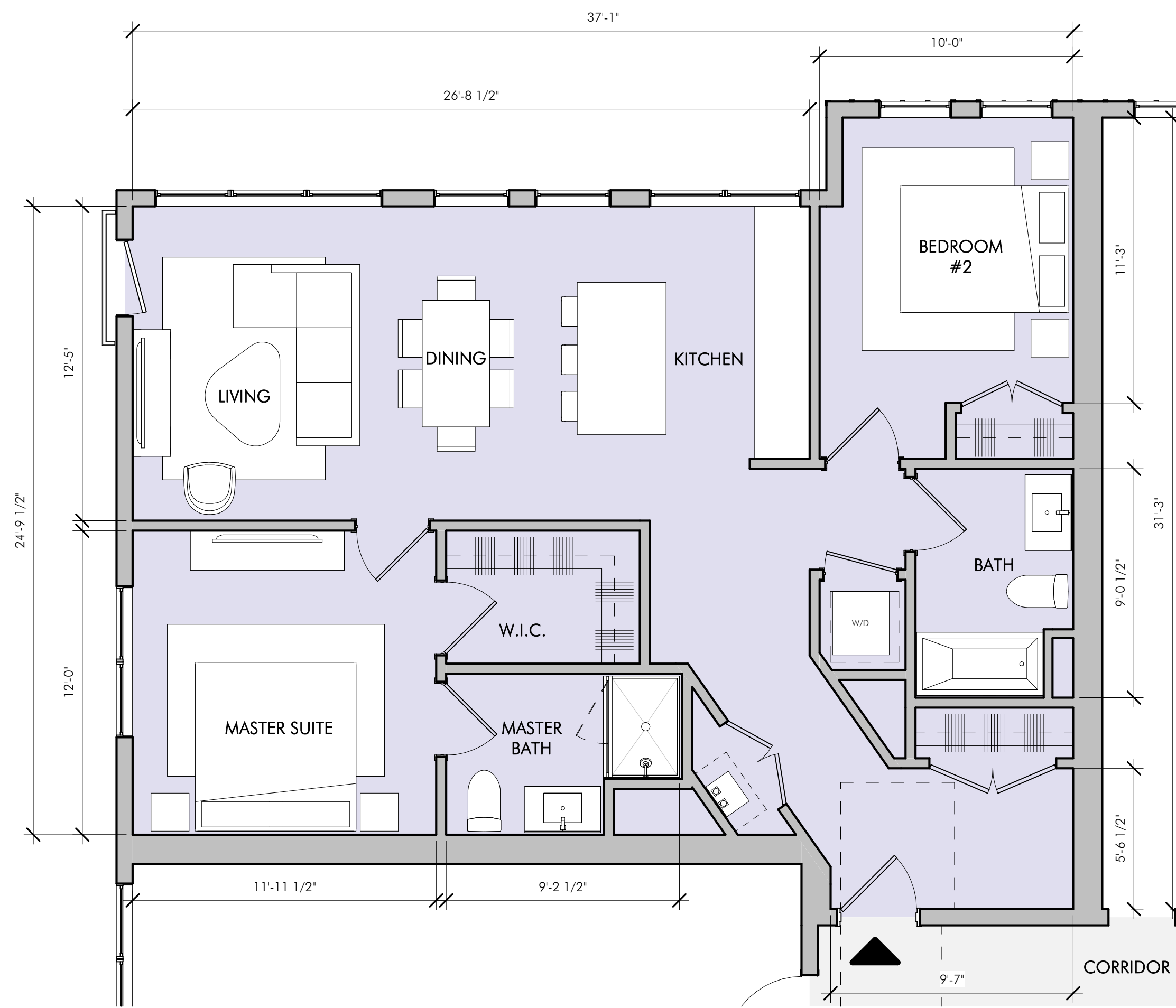
C TYPICAL 2 BEDROOM (1,035 SF) 1/4" = 1'-0"
