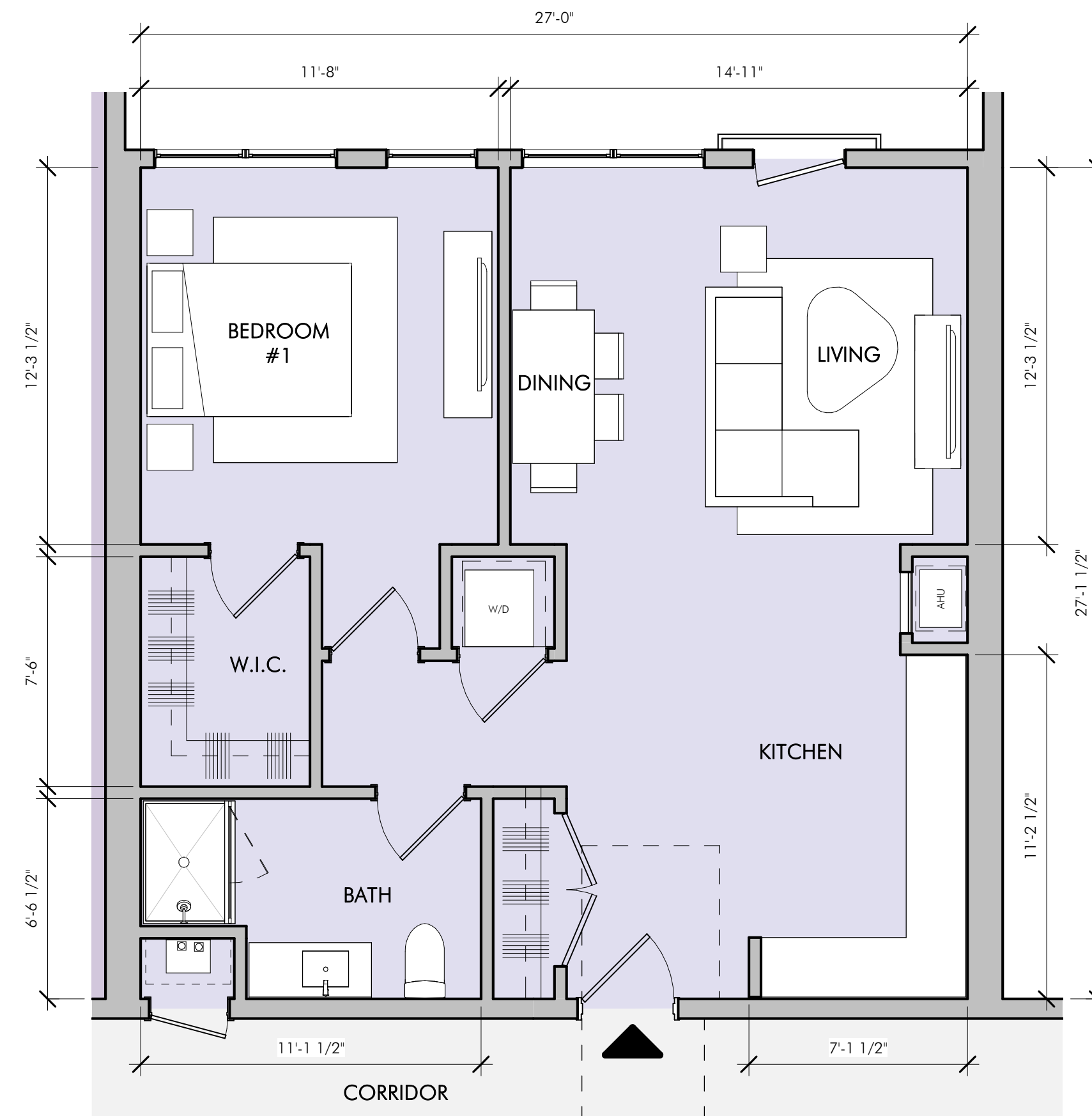
B TYPICAL 1 BEDROOM (775 SF) 1/4" = 1'-0"
