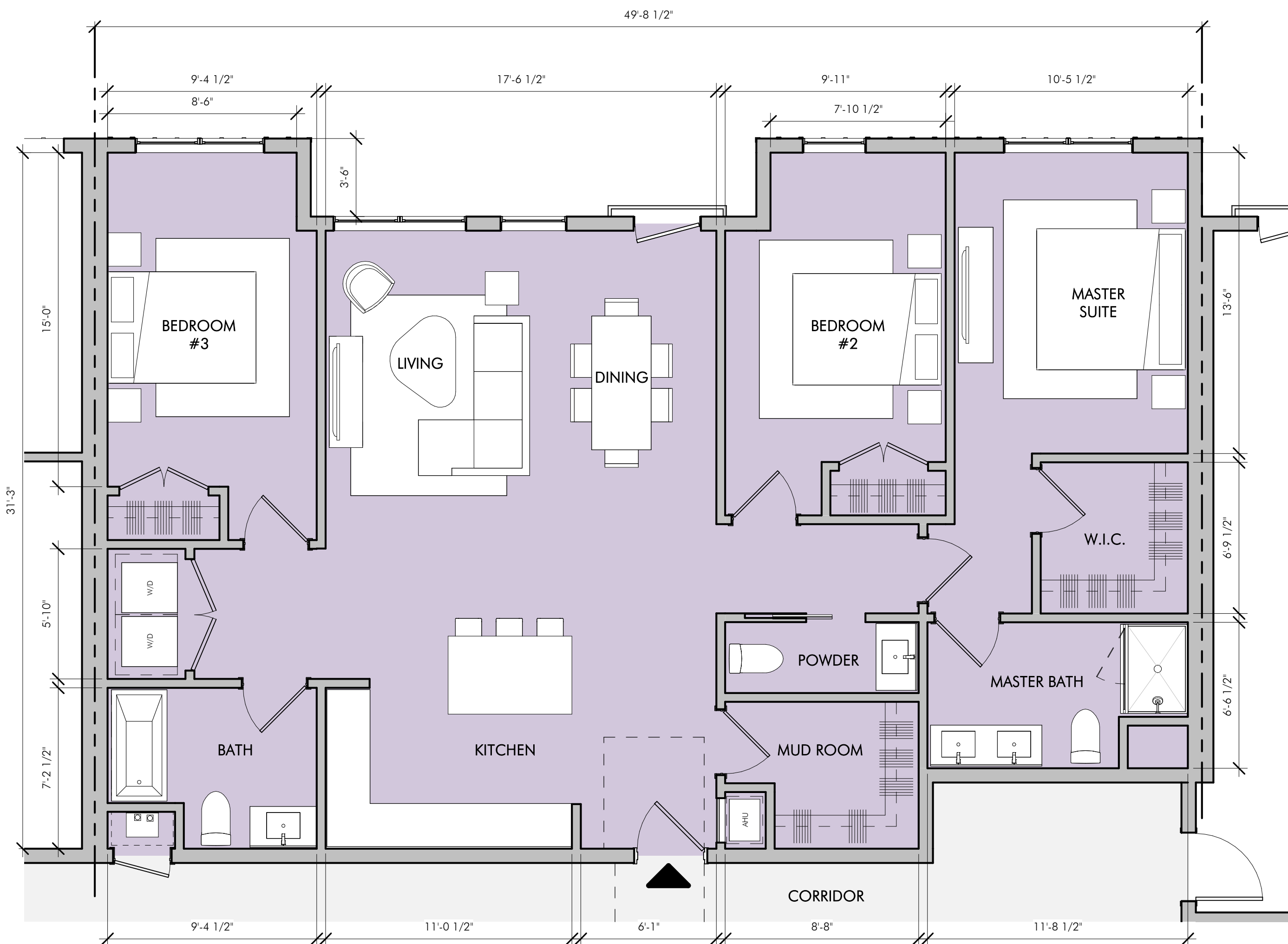
2 TYPICAL 3 BEDROOM (1,460 SF) 1/4" = 1'-0"
